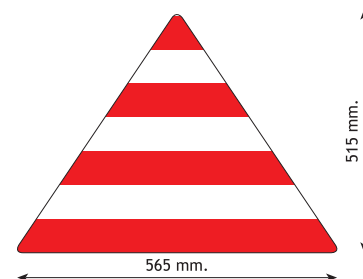
Cod. 70060 Aluminium triangle panel with reflecting film class 1. 565x515x2 mm.
