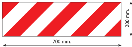
Cod. 80961 Kit aluminium panel white reflecting and red fluorescent. 700x200x2 mm.
